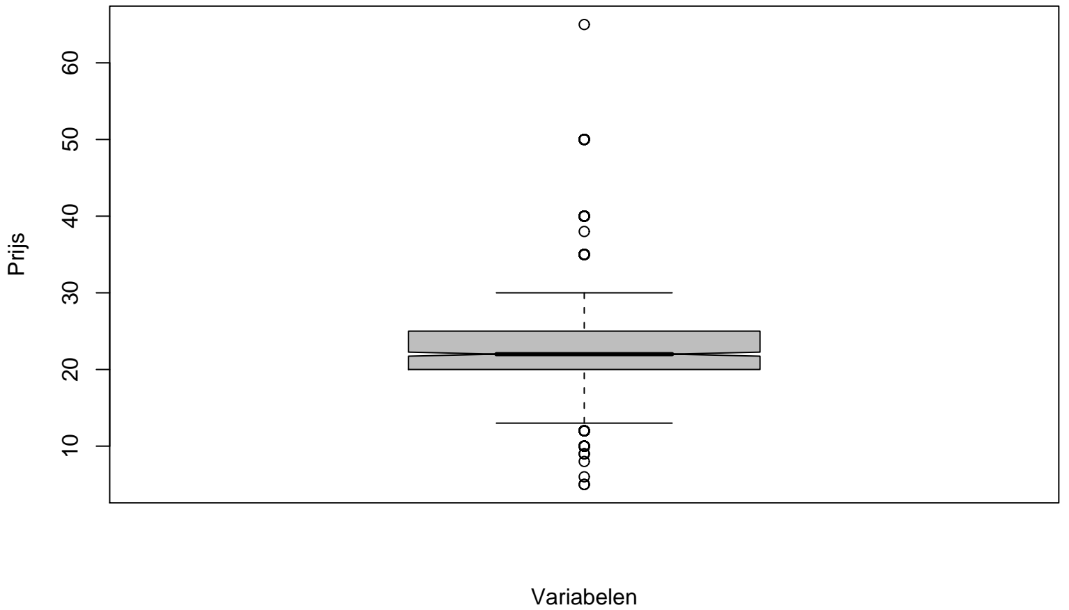
Box plot studio 100
