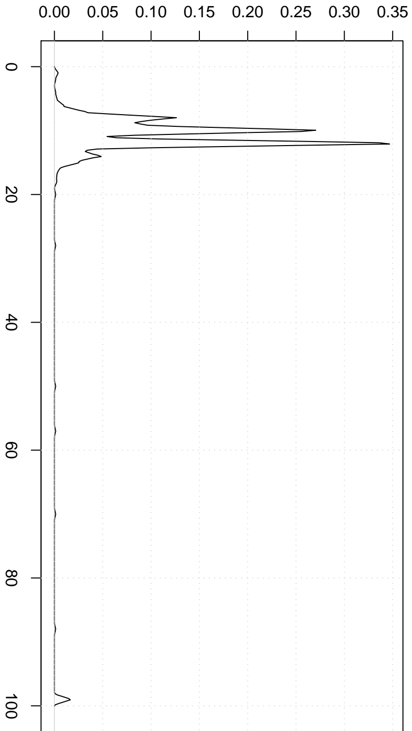
Triangular Kernel
