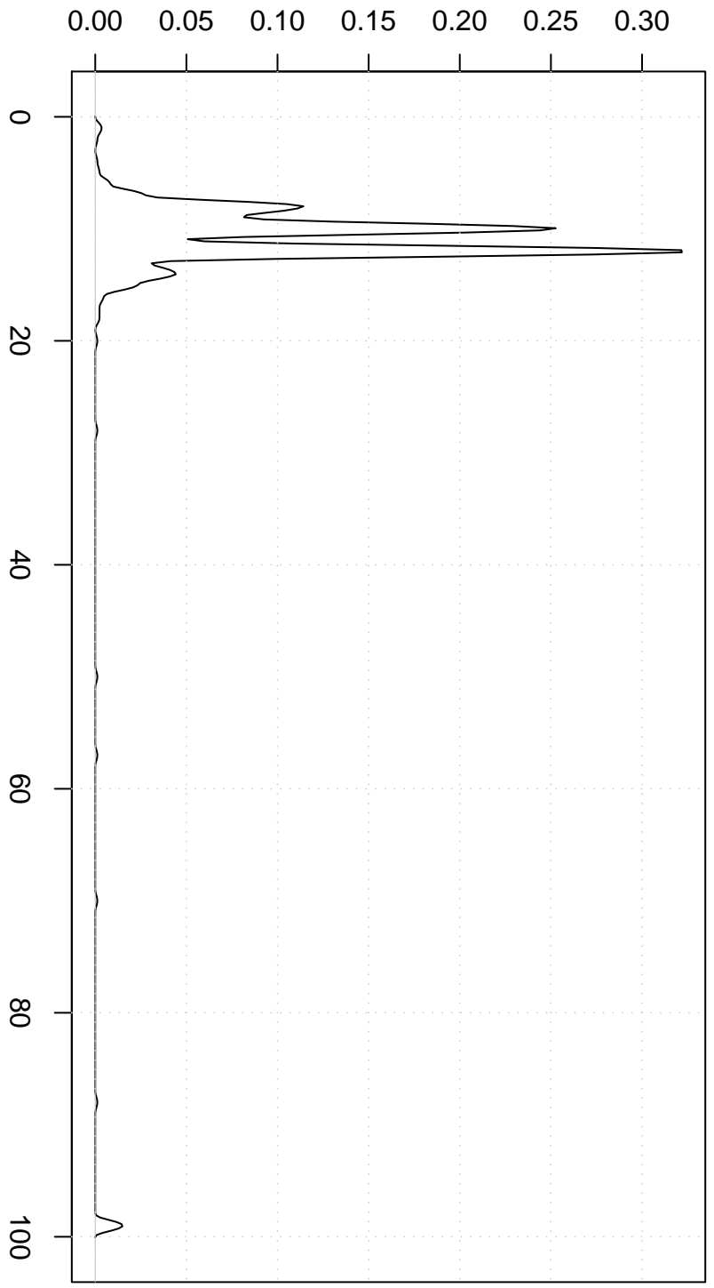
Biweight Kernel
