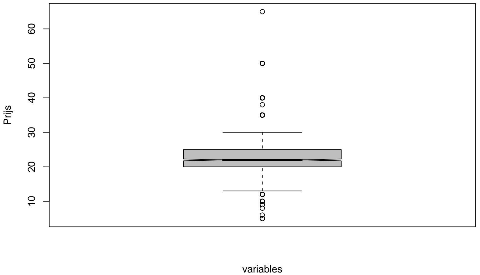
Boxplot Studio 100
