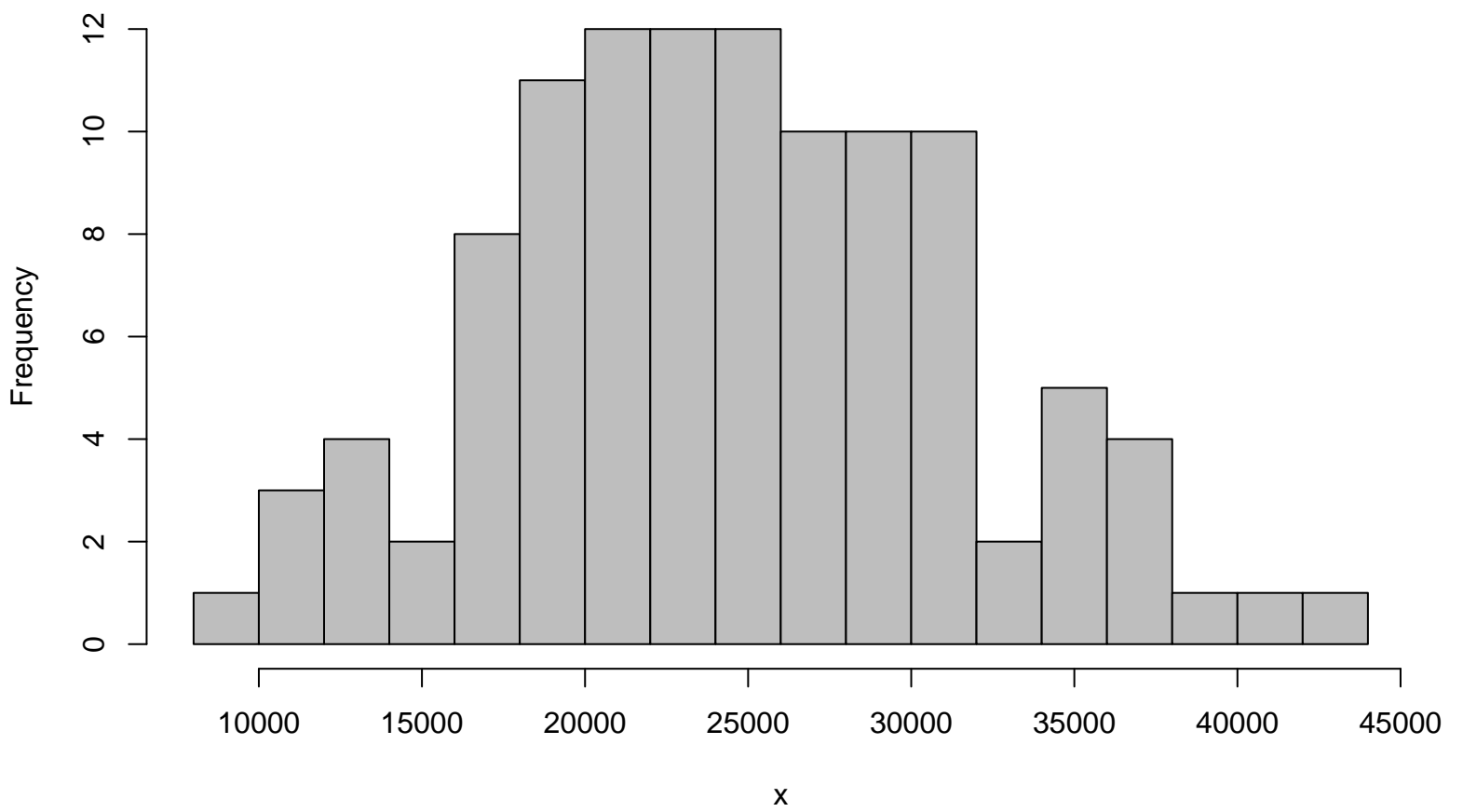
Histogram
