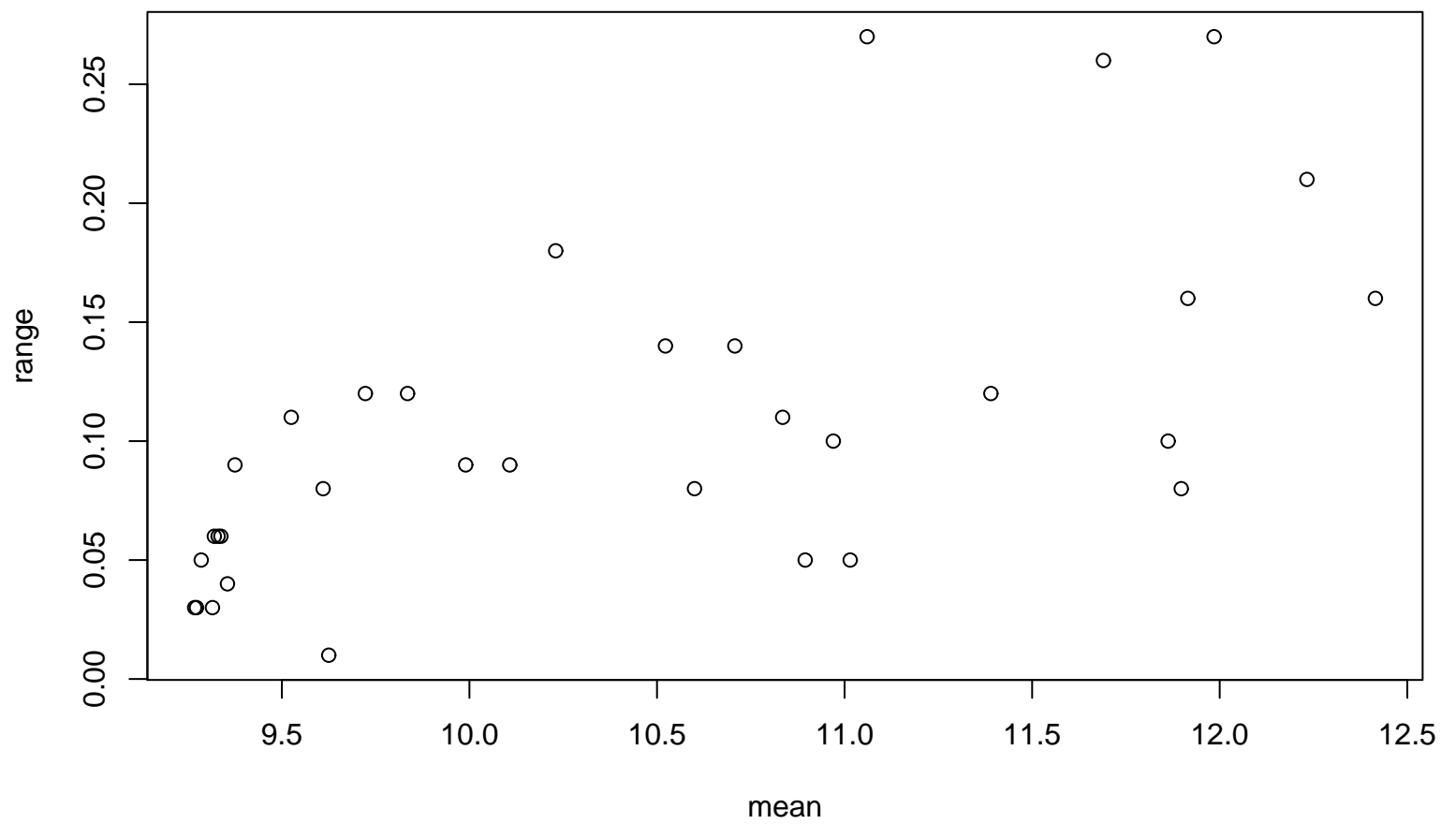
Range–Mean Plot
