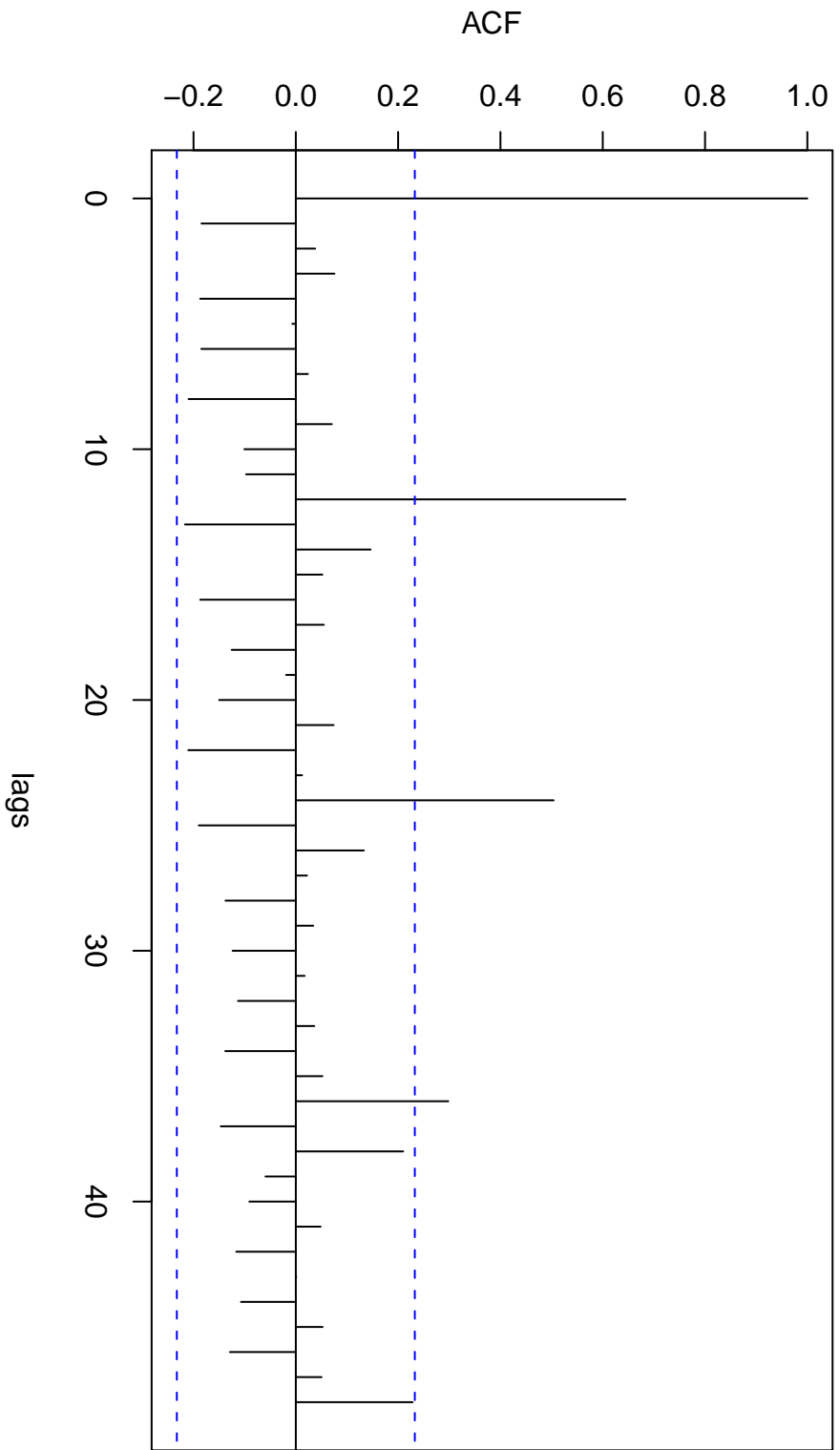
Autocorrelation
