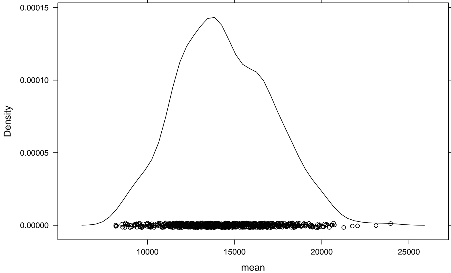
Density Plot
