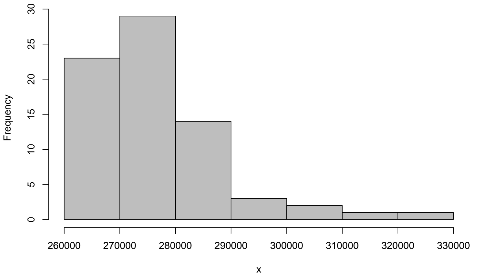
Histogram
