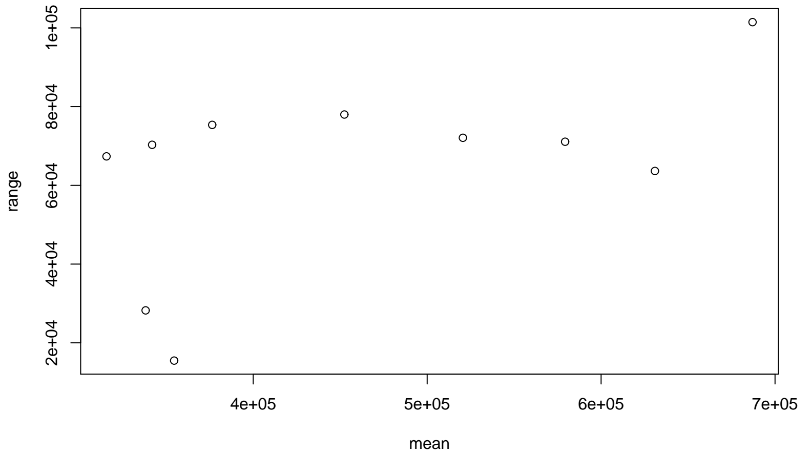
Range–Mean Plot
