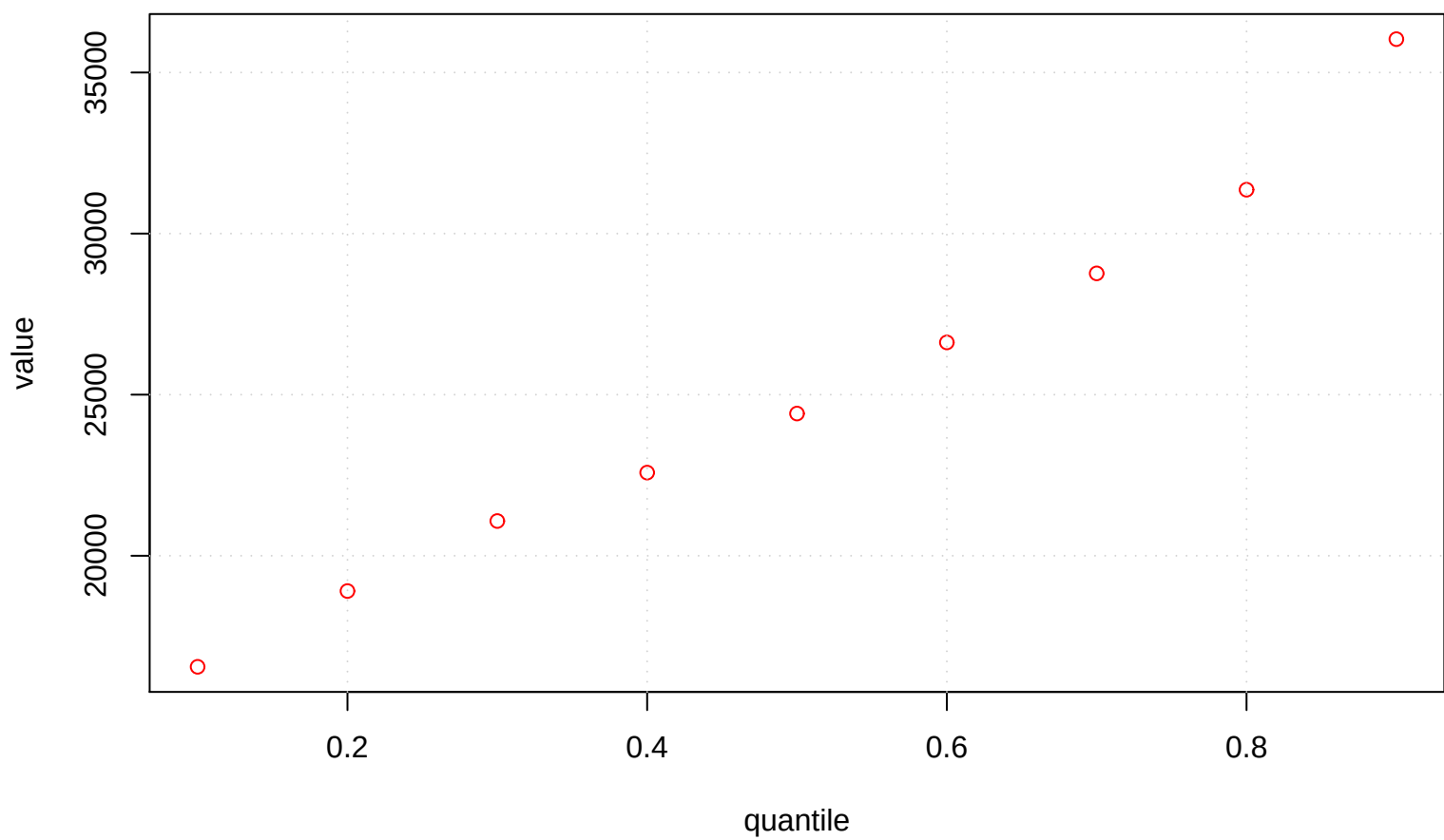
Harrell-Davis Quantiles
