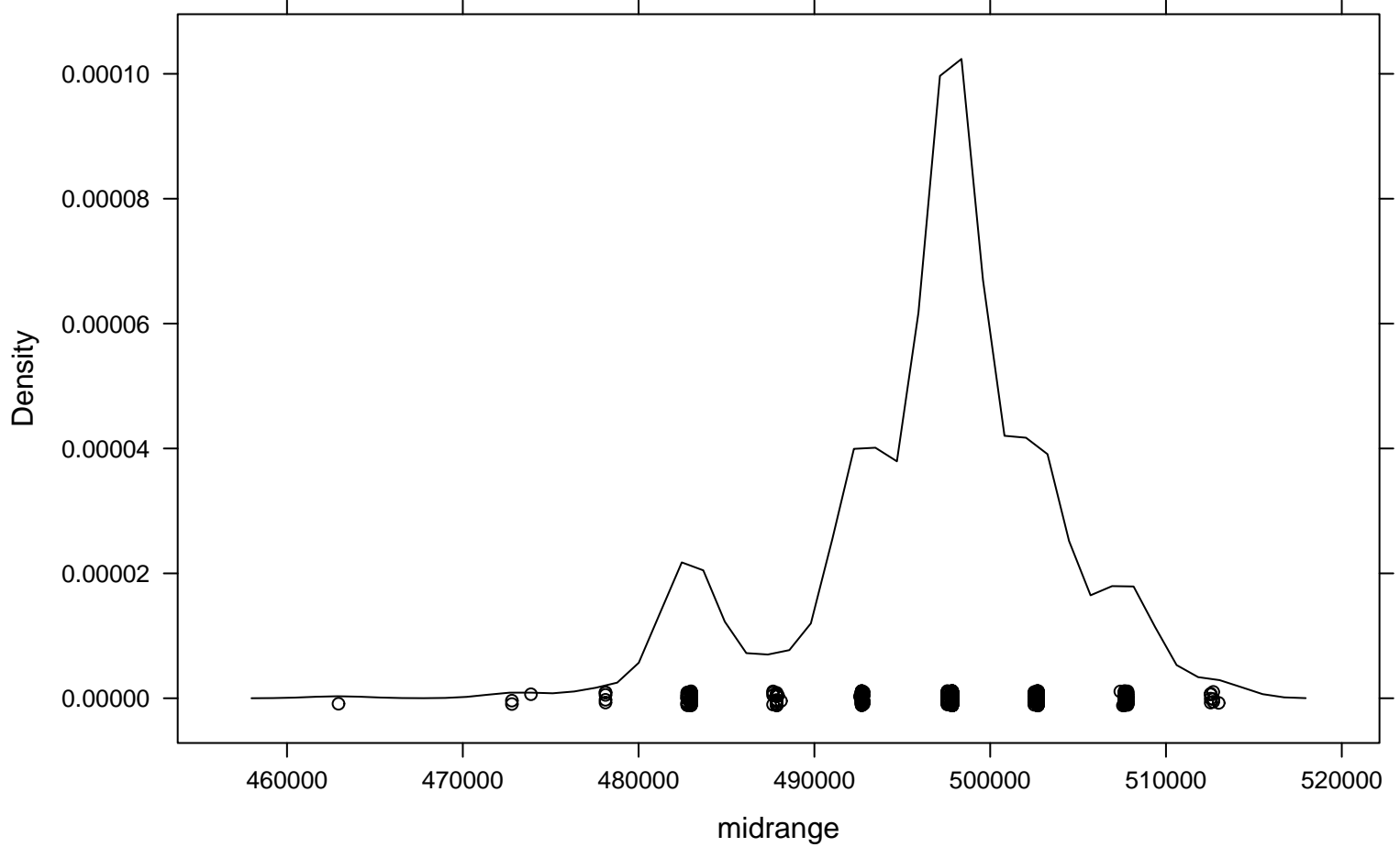
Density Plot
