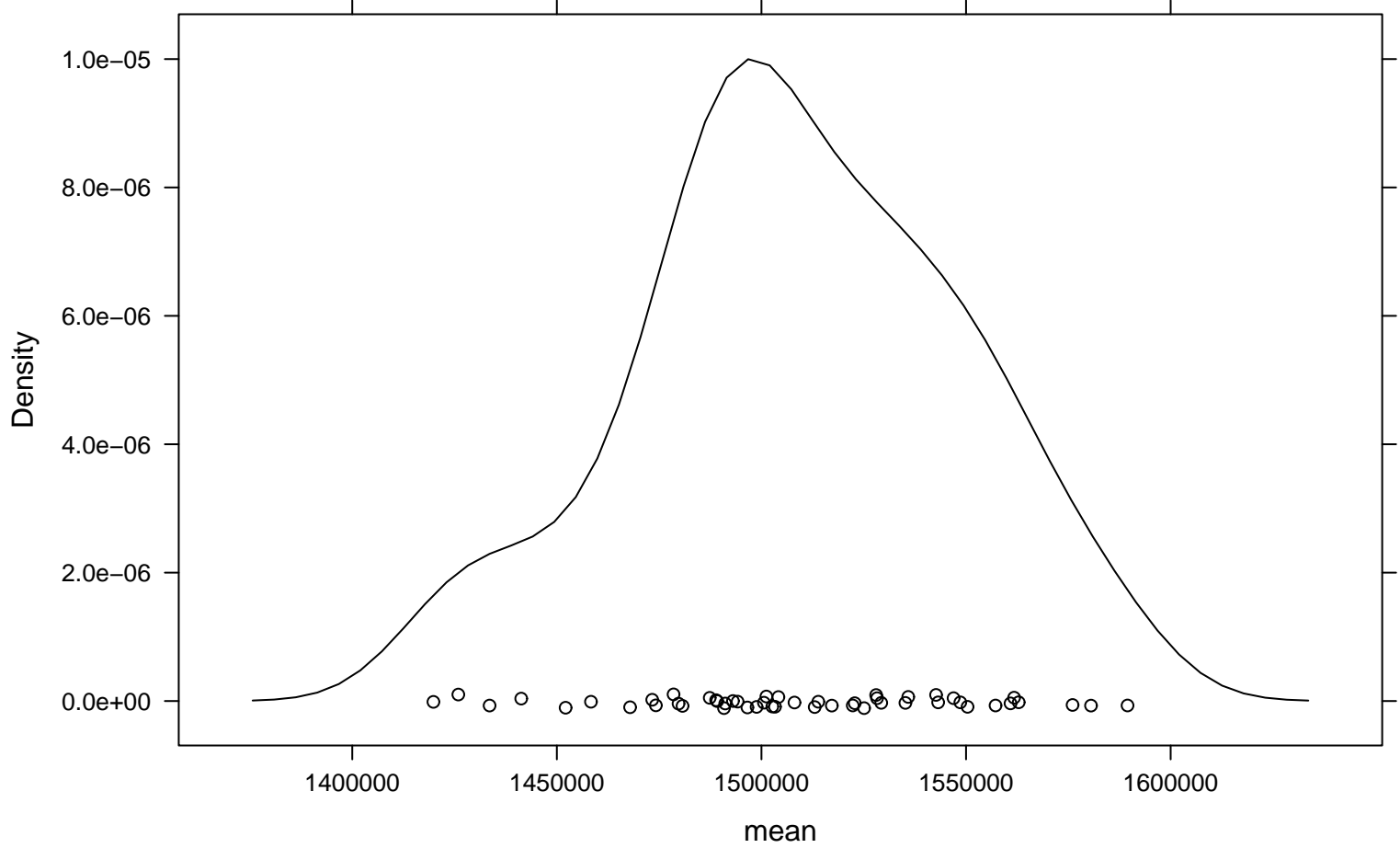
Density Plot
