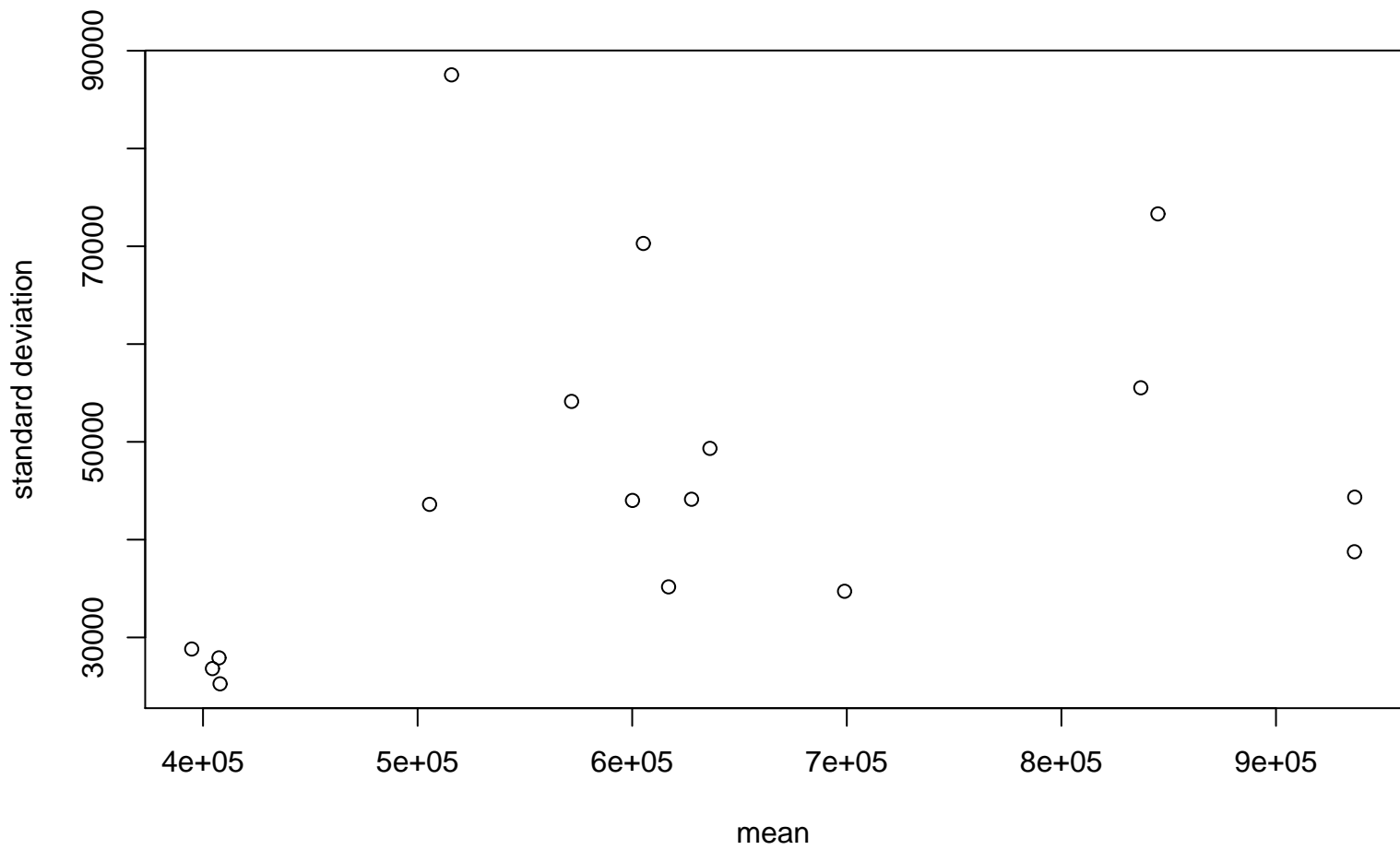
Standard Deviation–Mean Plot
