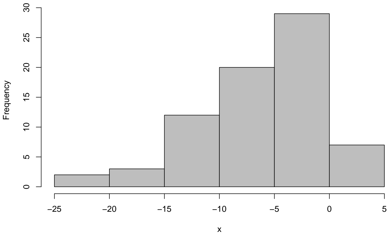
Histogram
