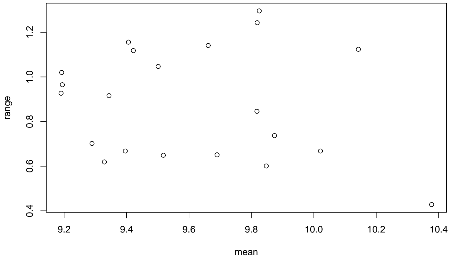
Range–Mean Plot
