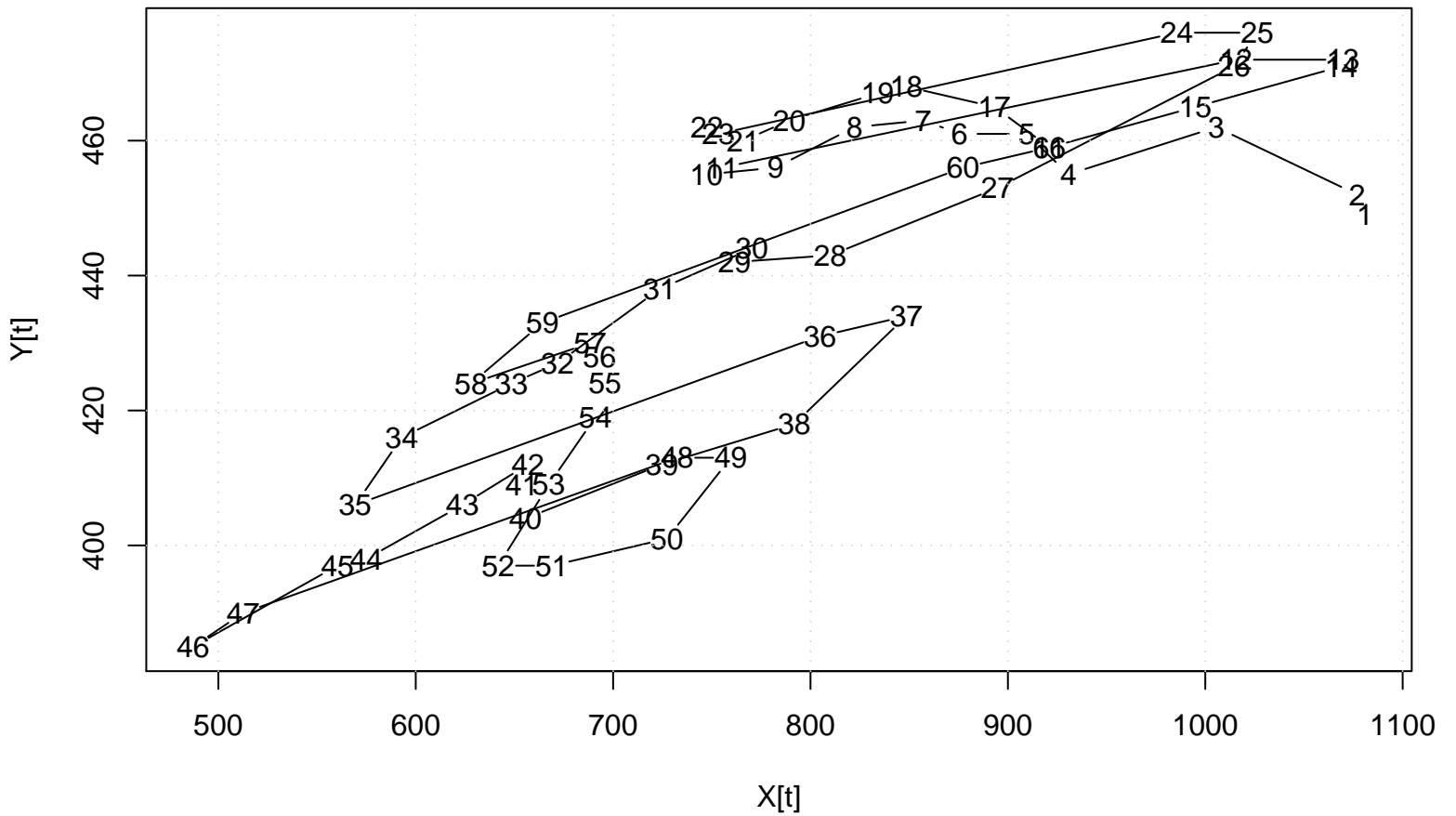
Scatter Plot
