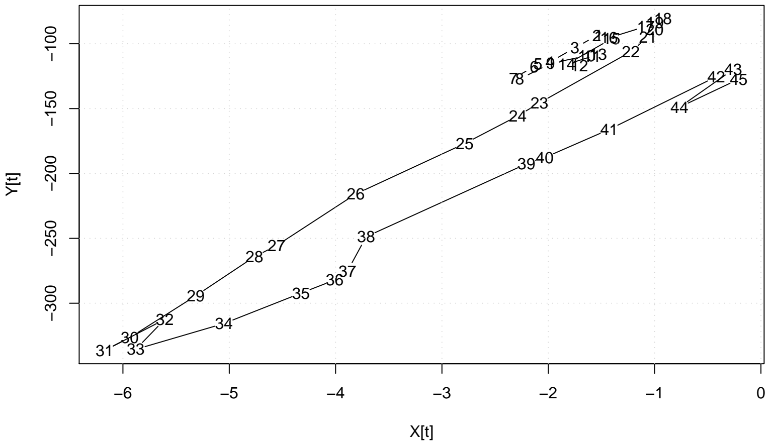
Scatter Plot
