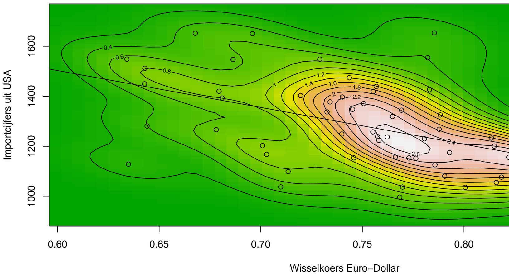
Bivariate Kernel Density Plot (x,y)
