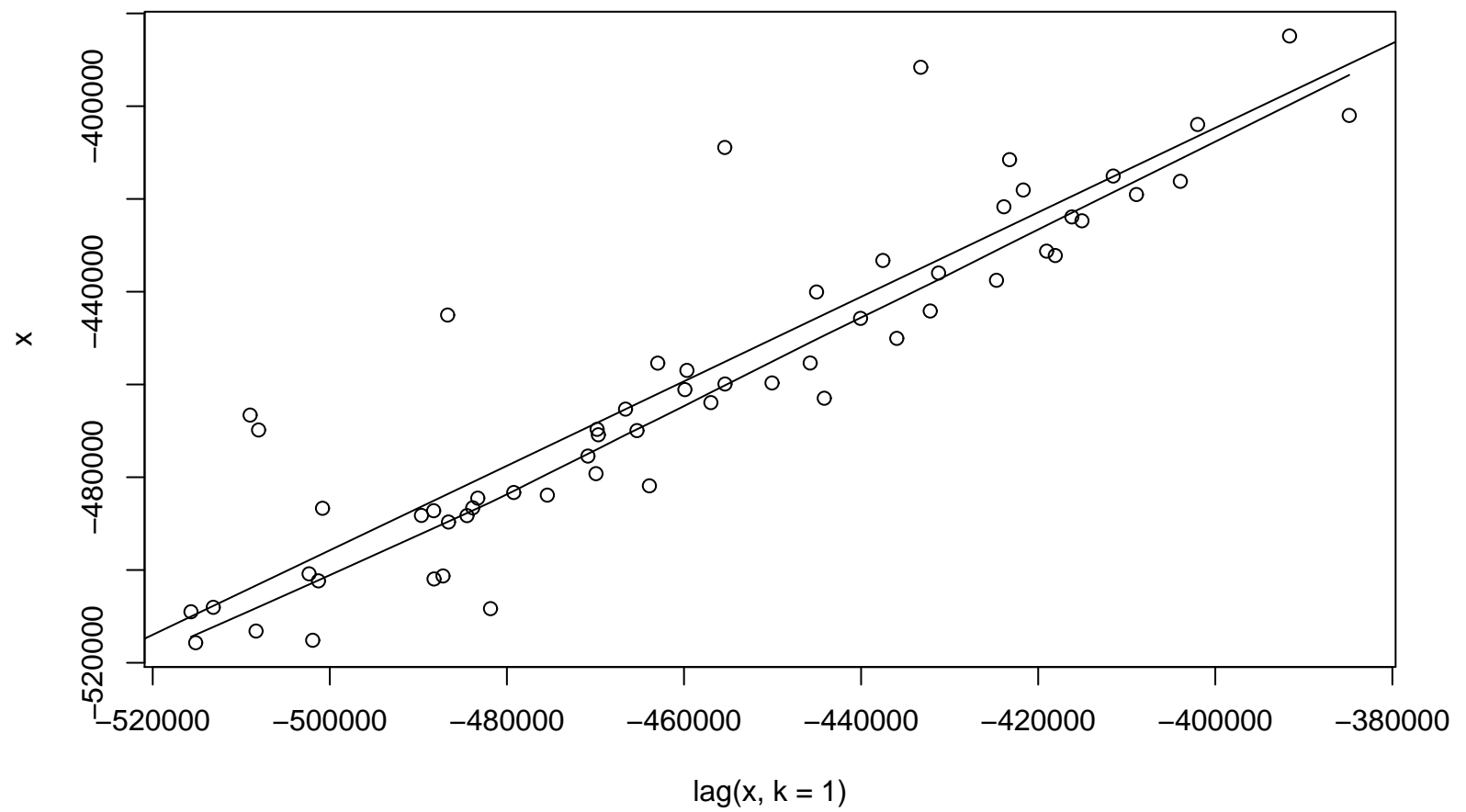
Lag plot (k=1), lowess, and regression line
