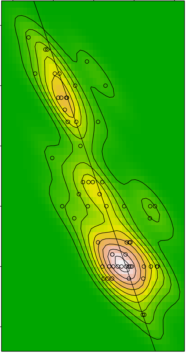
Bivariate Kernel Density Plot (y,z)
