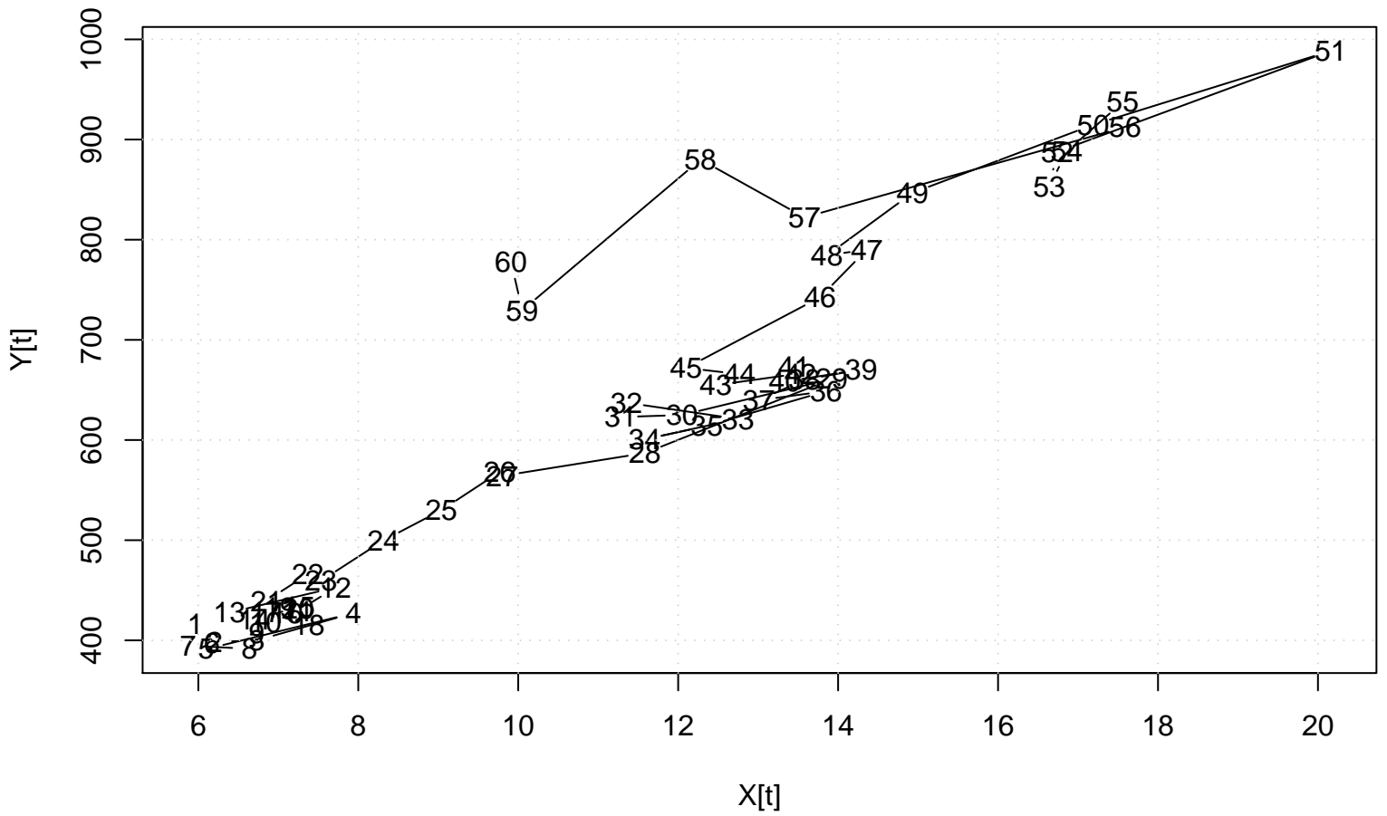
Scatter Plot
