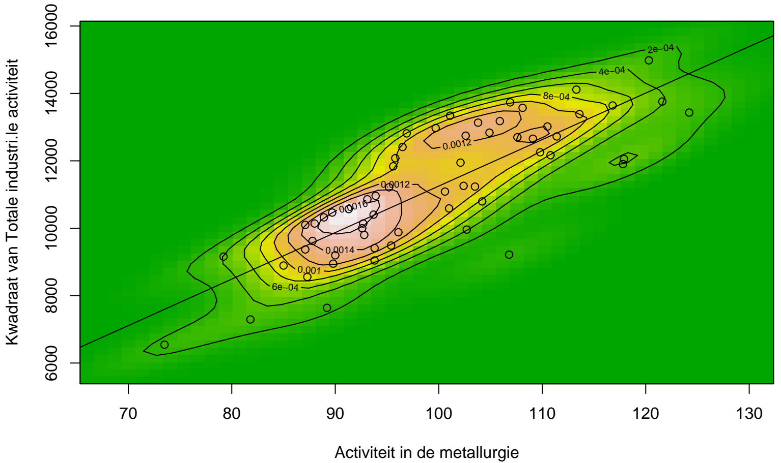
Bivariate Kernel Density Plot (x,y)
