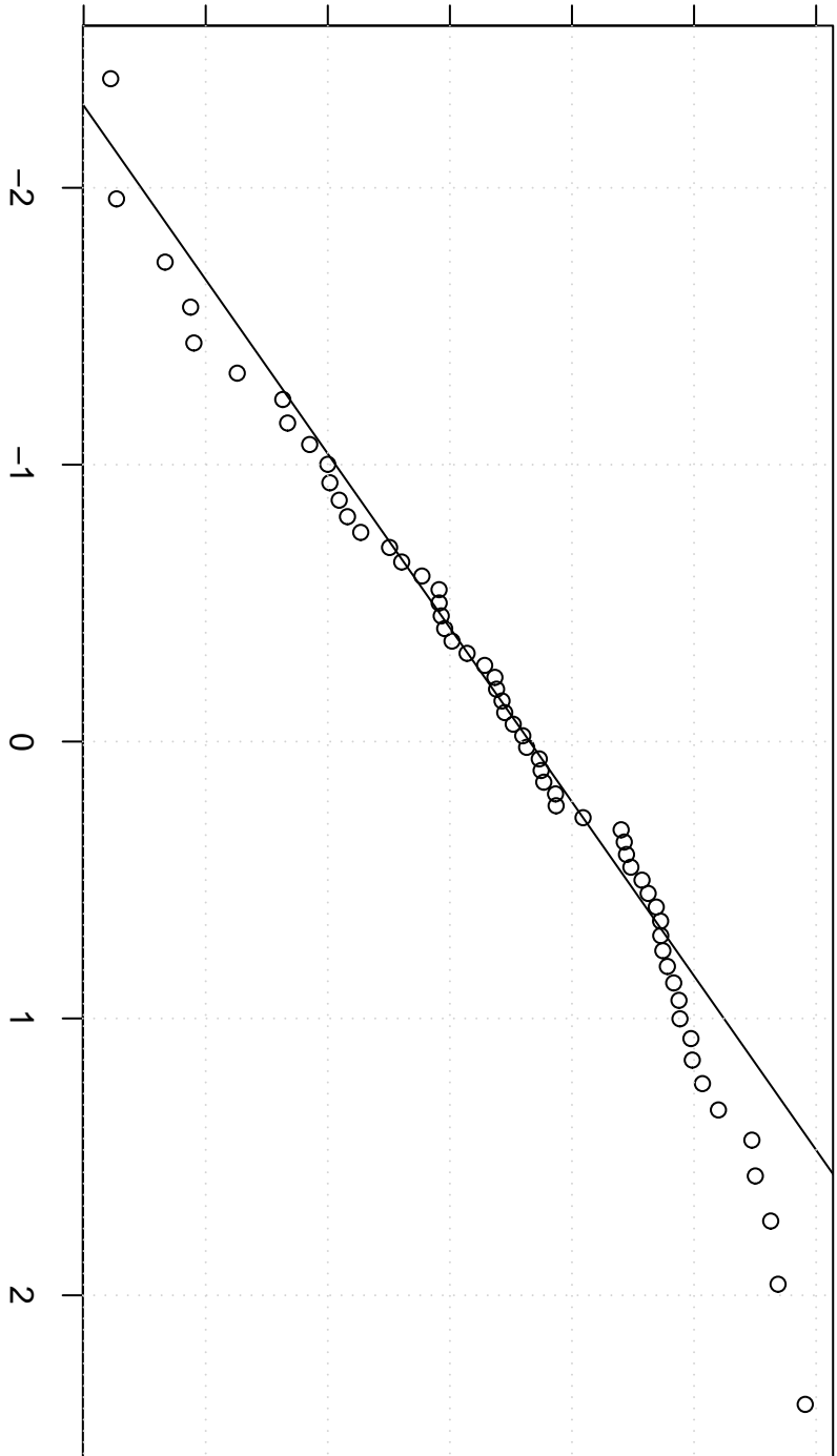
Theoretical Quantiles
