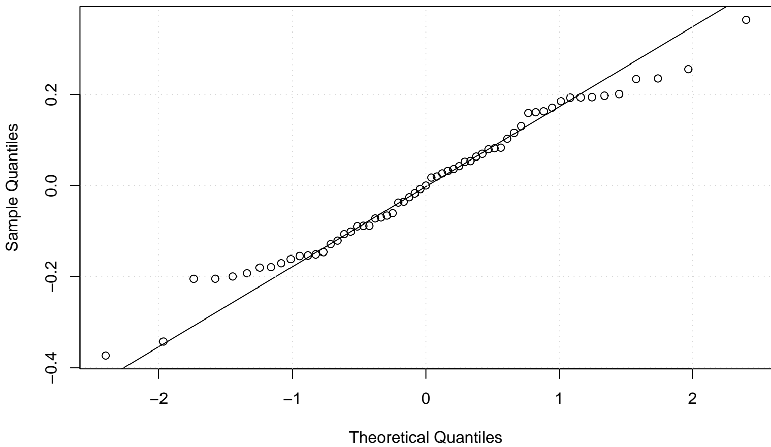
QQ plot of e[t]
