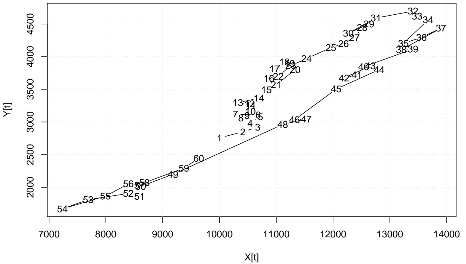
Scatter Plot
