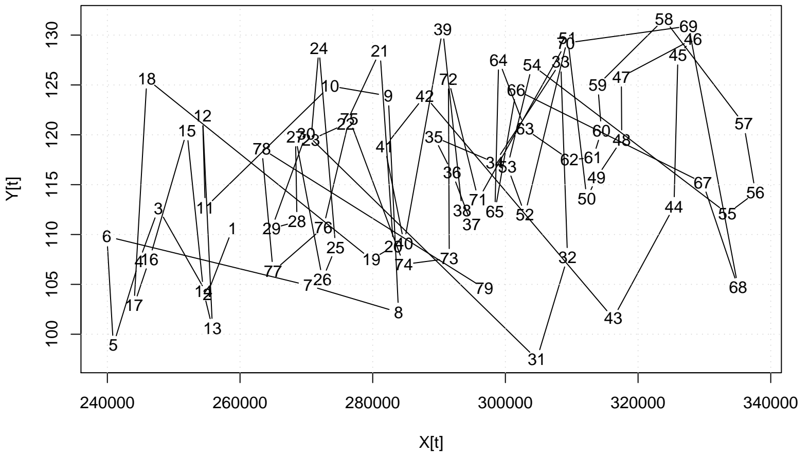
Scatter Plot
