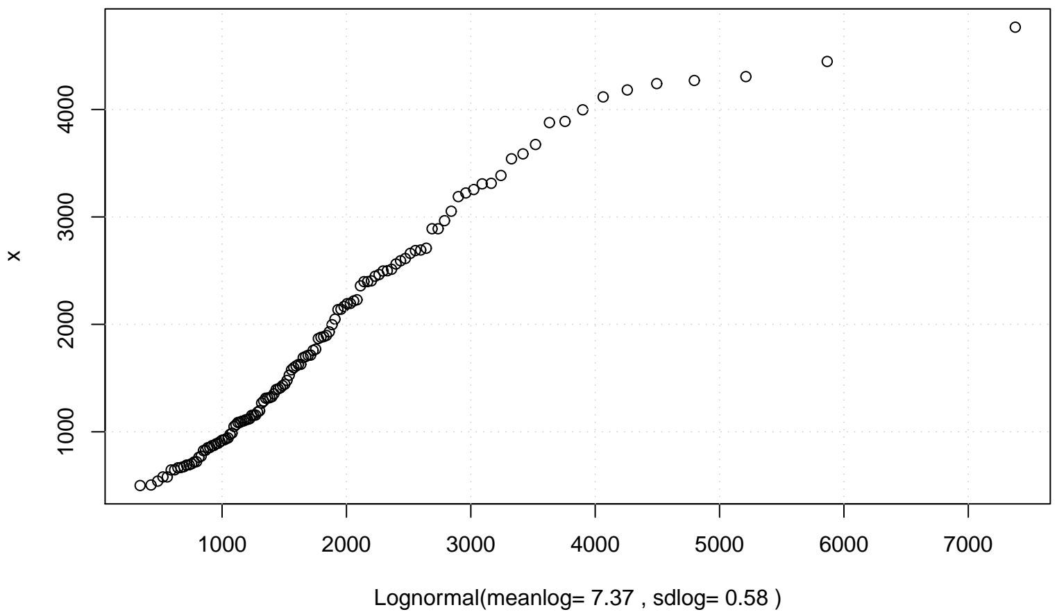
QQ plot (Lognormal)
