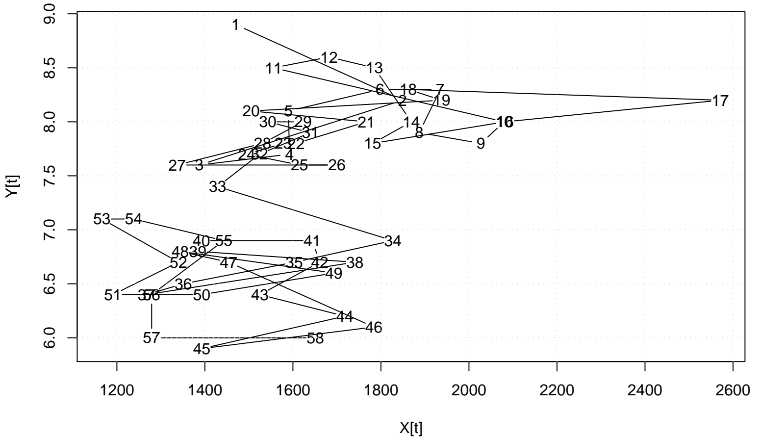
Scatter Plot
