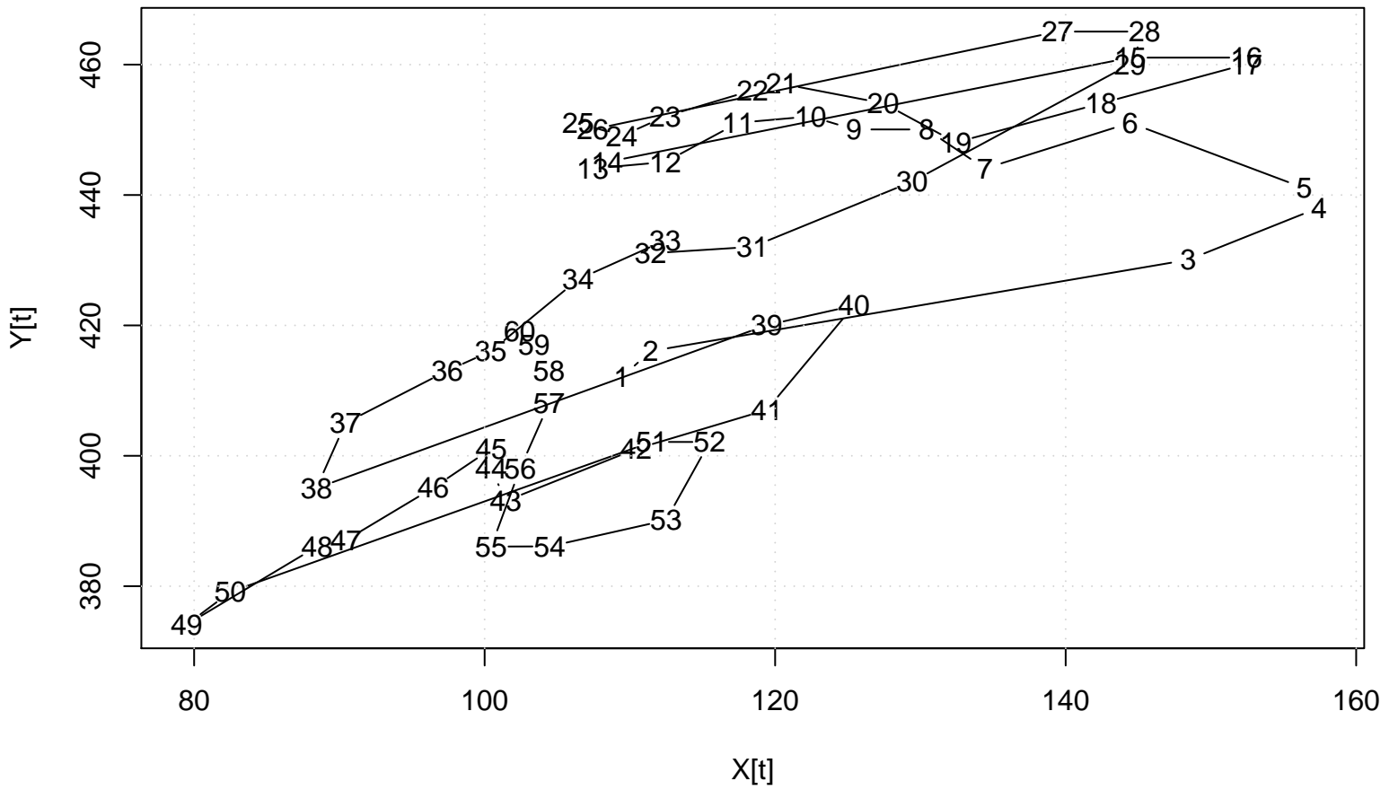
Scatter Plot
