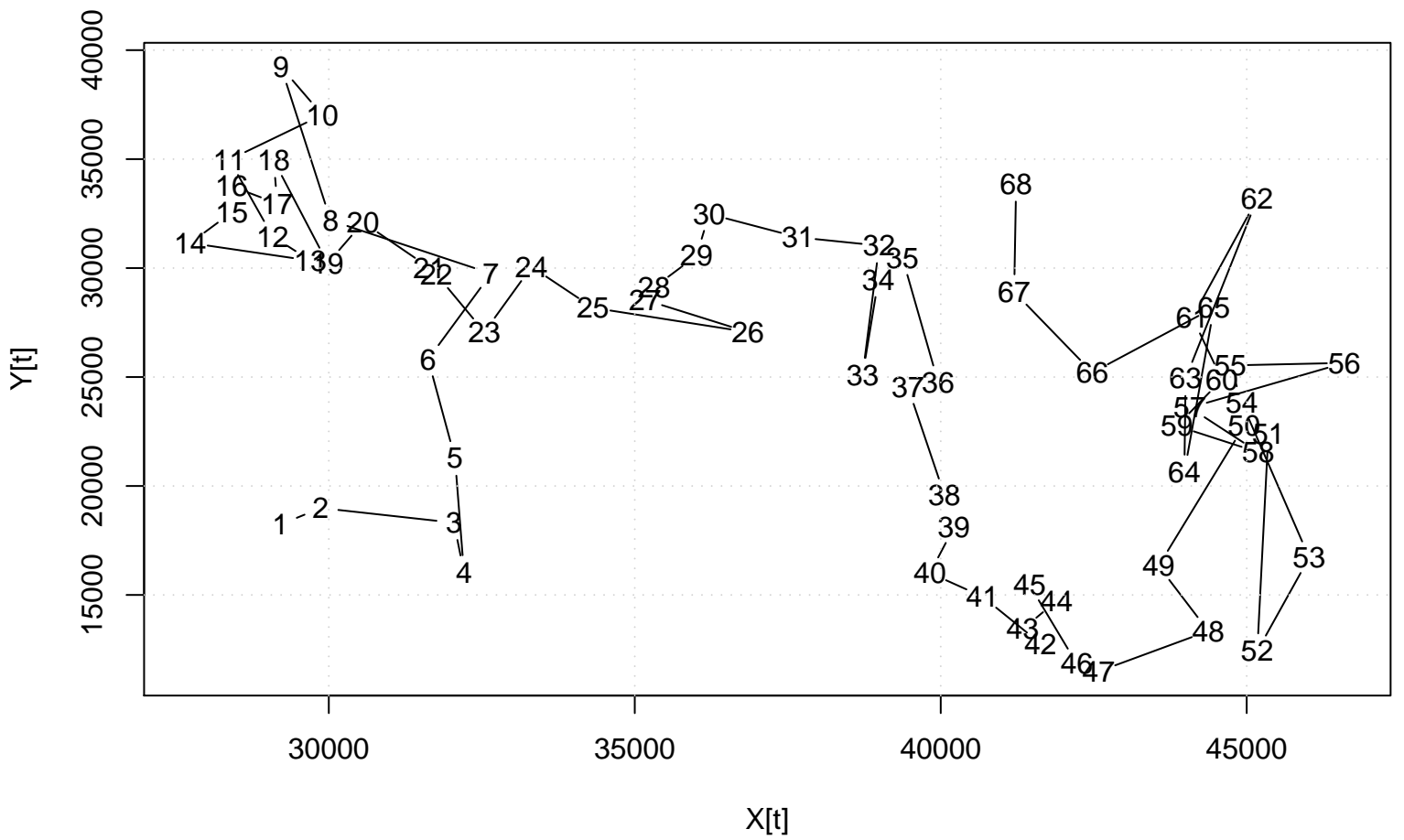
Scatter Plot
