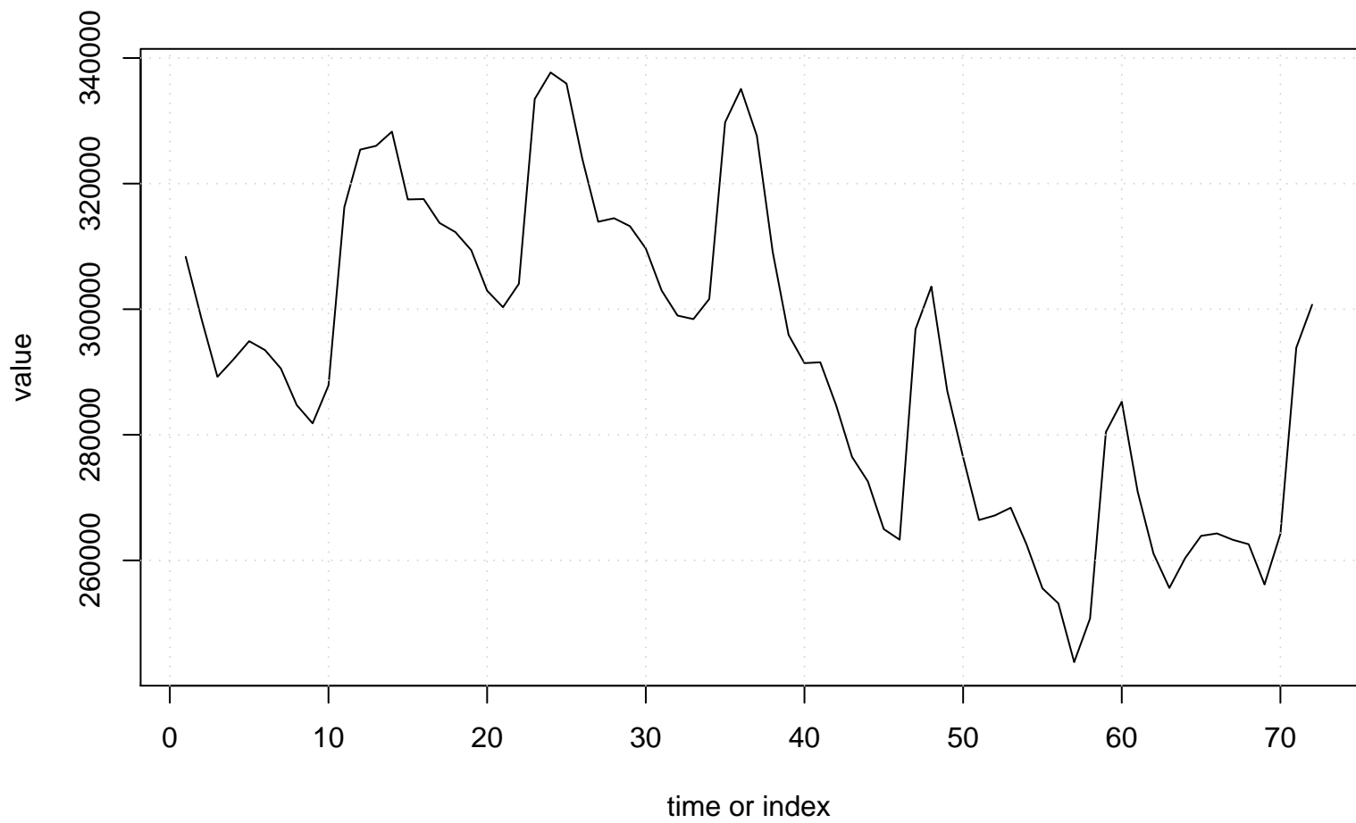
Run Sequence Plot of Y[t]
