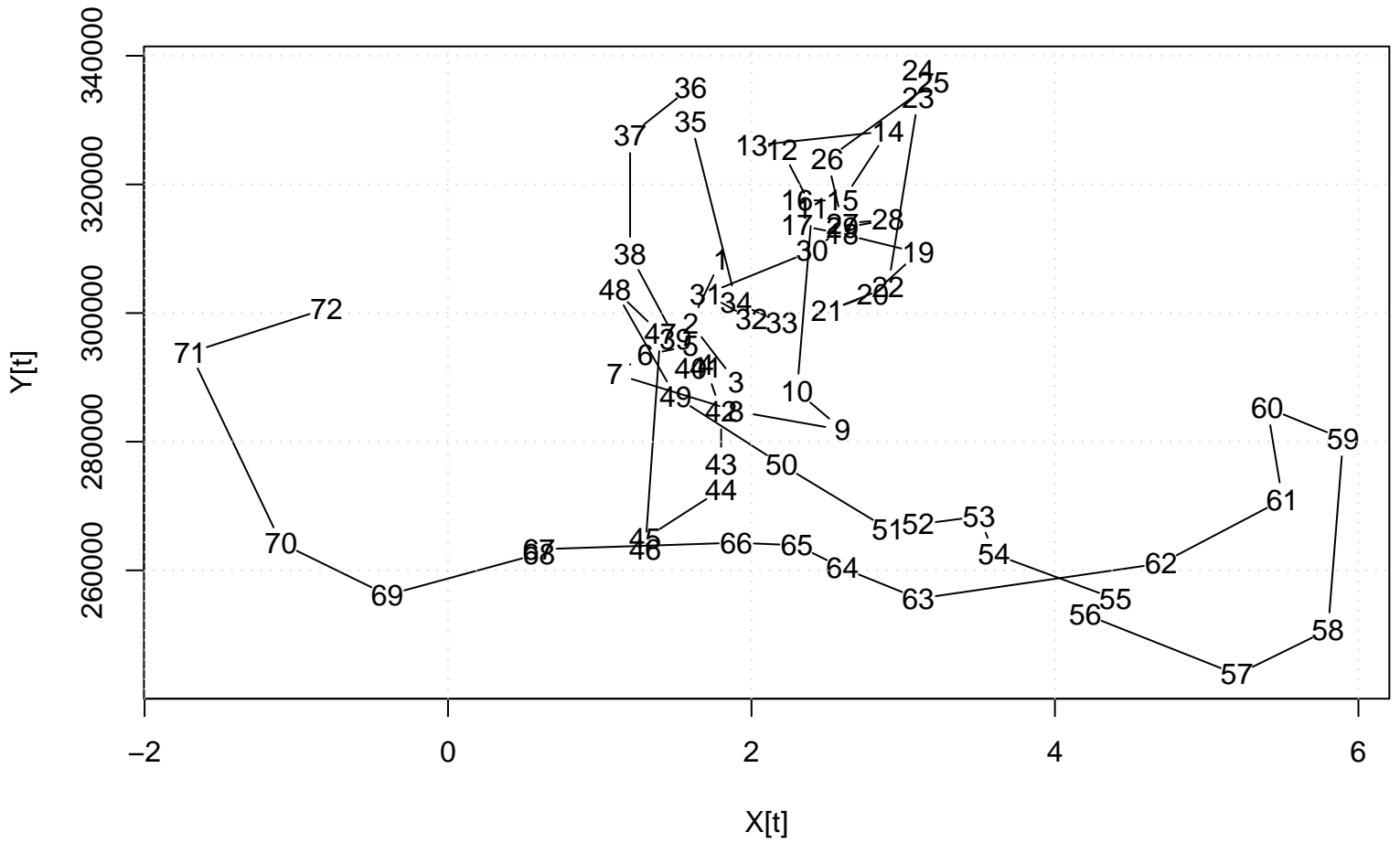
Scatter Plot
