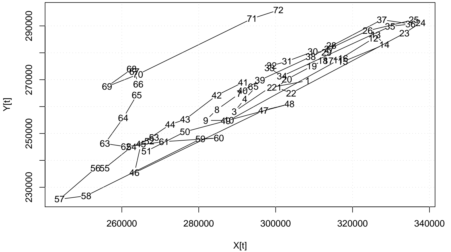
Scatter Plot
