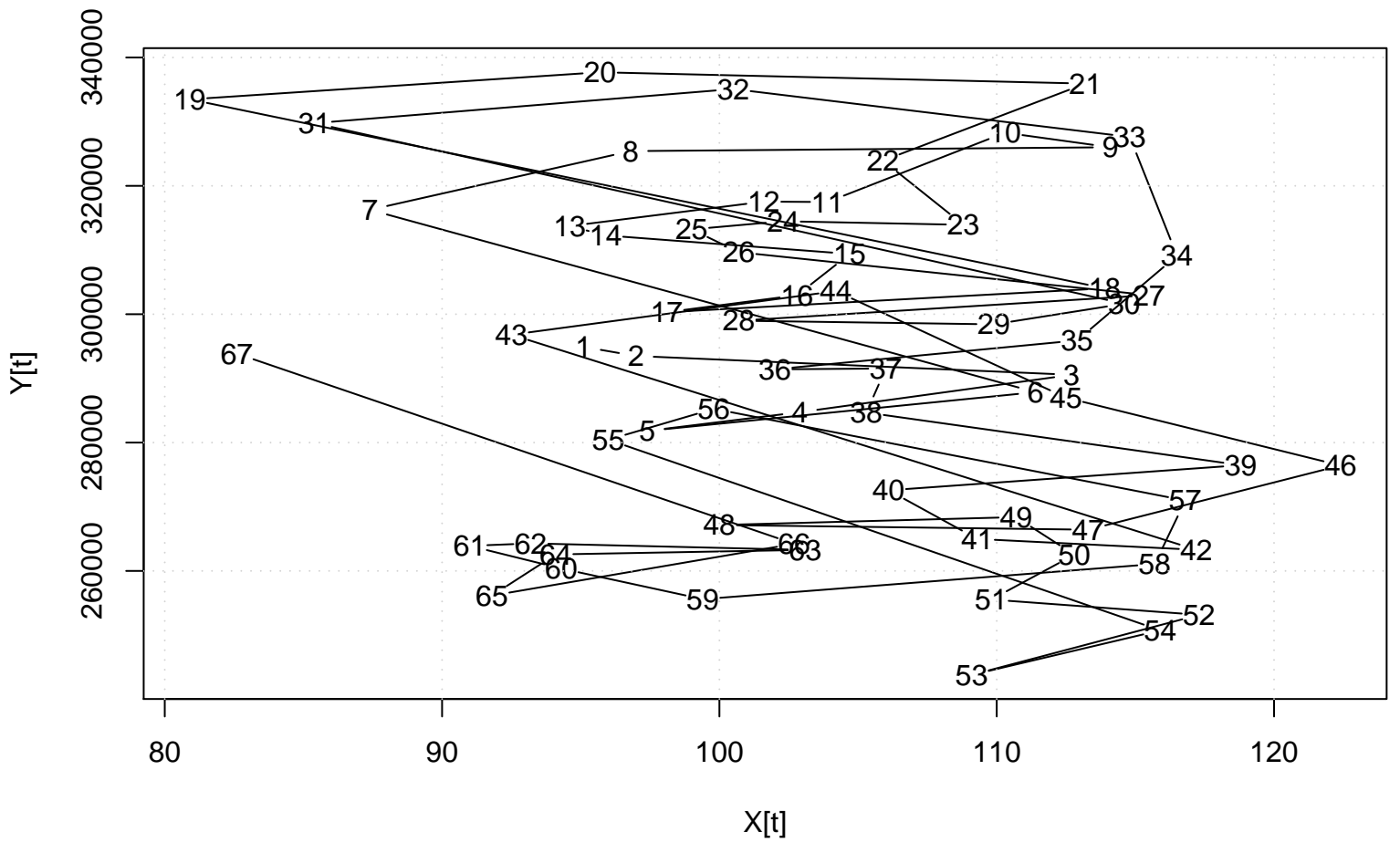
Scatter Plot
