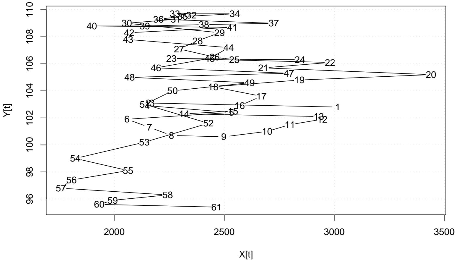
Scatter Plot
