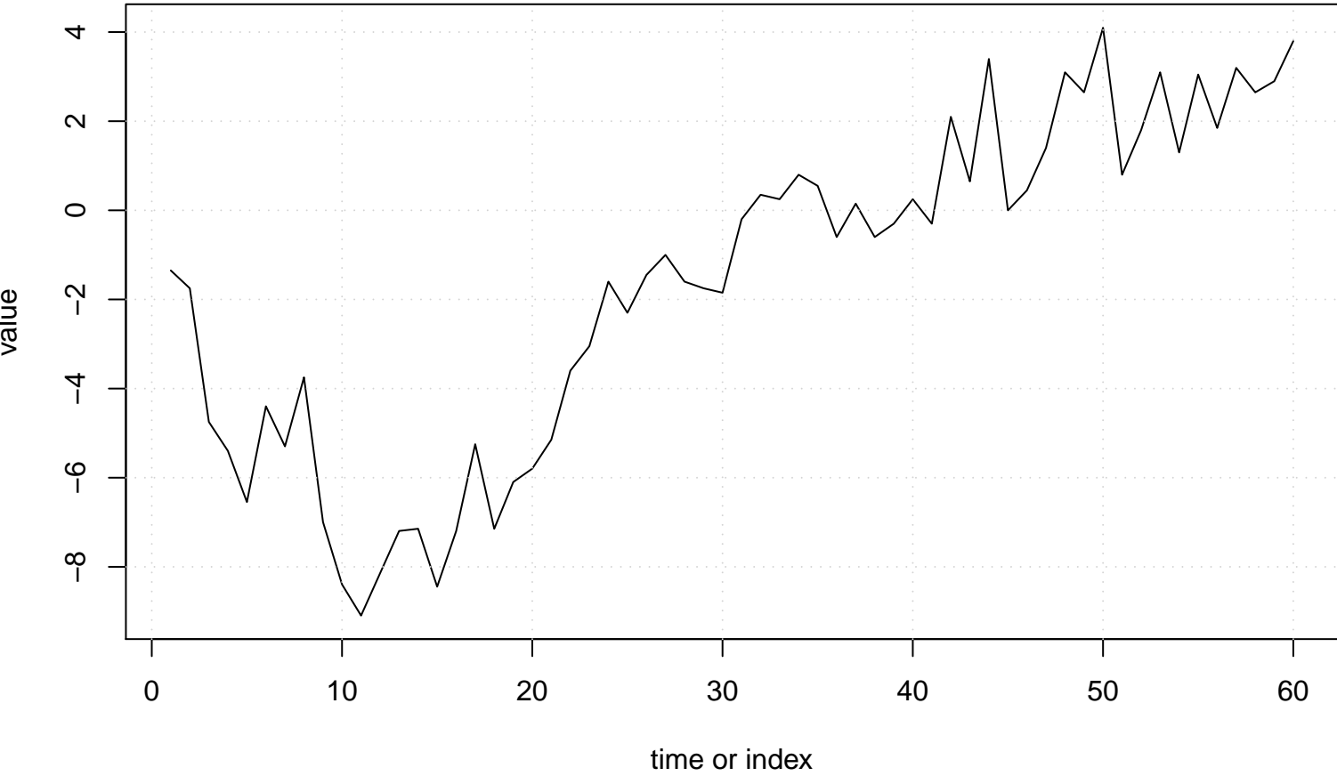
Run Sequence Plot of X[t]
