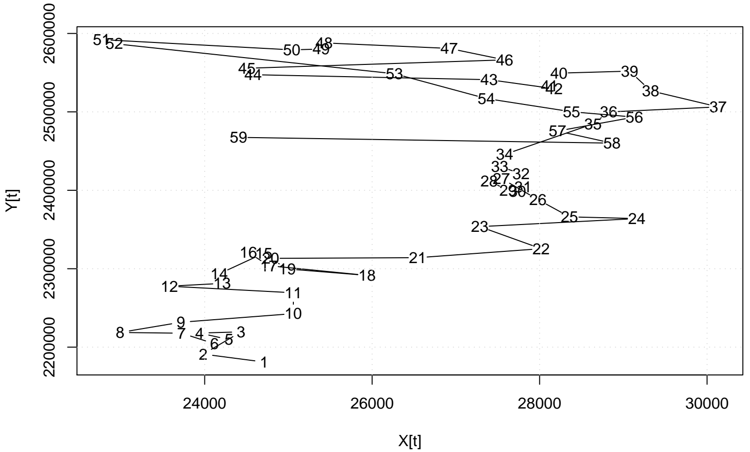
Scatter Plot
