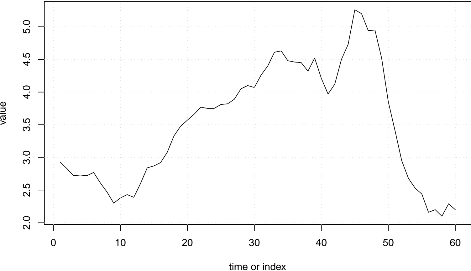
Run Sequence Plot of Y[t]
