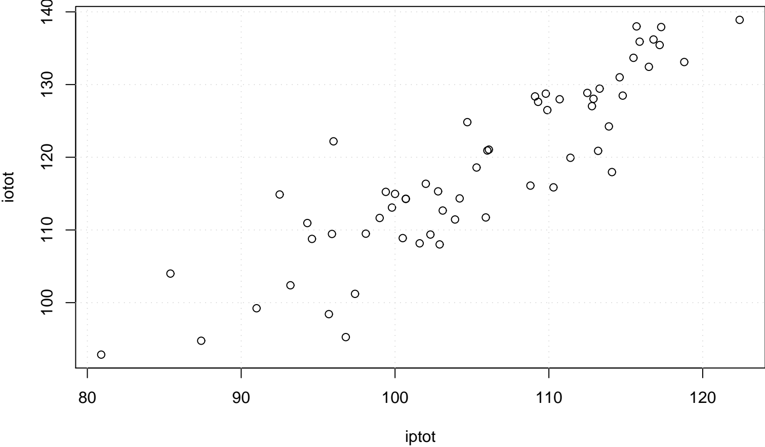
Scatterplot
