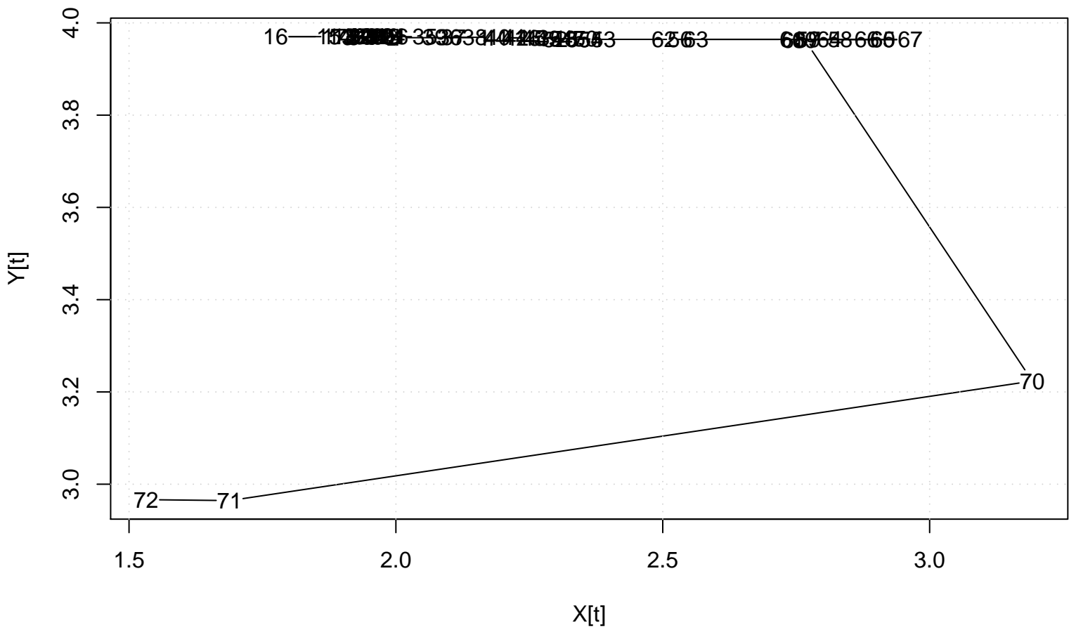
Scatter Plot
