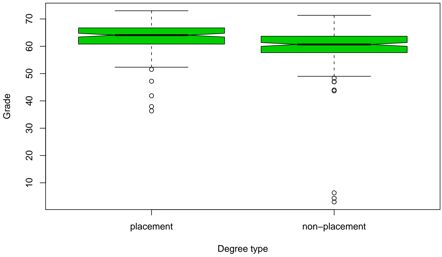
Boxplot week 5 – Reddy and Moores
