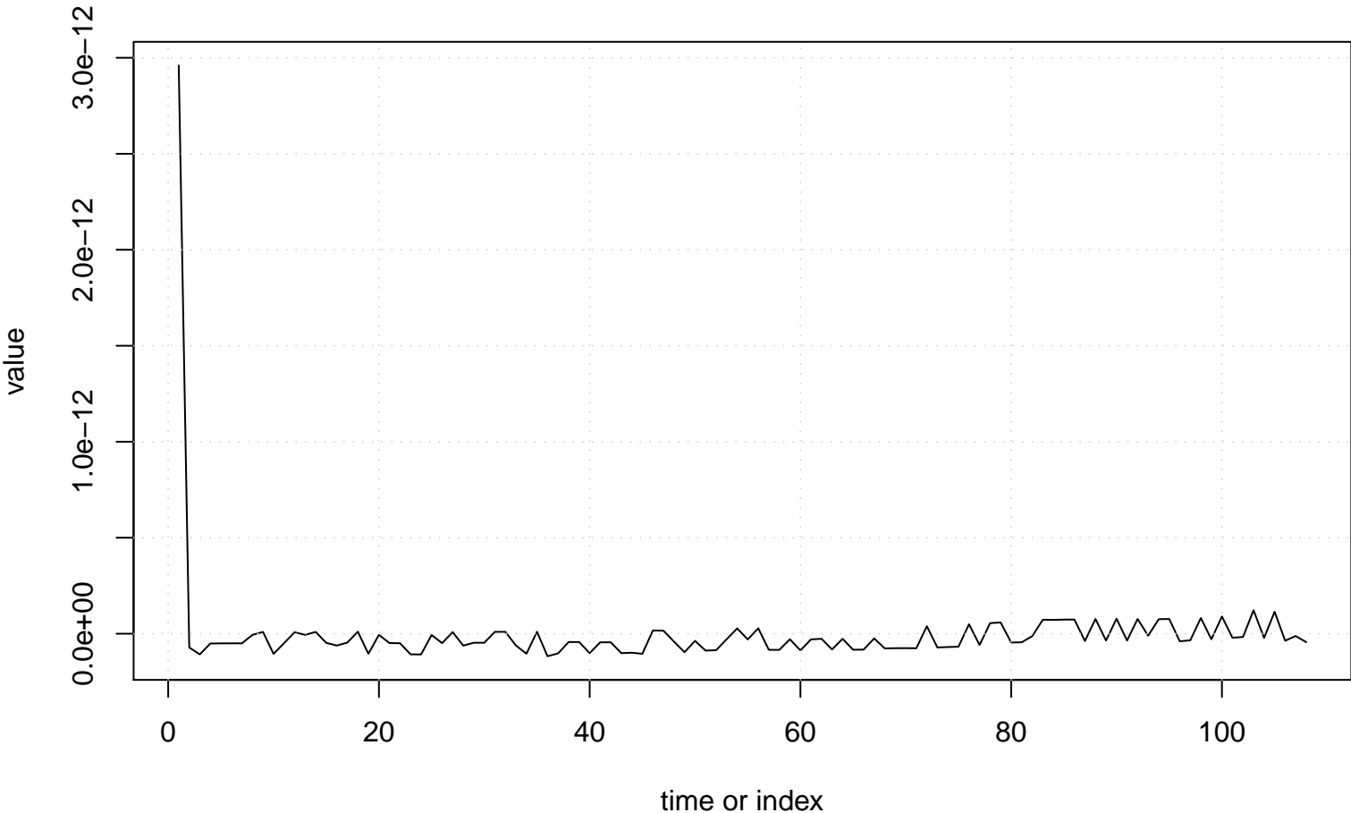
Run Sequence Plot of e[t]
