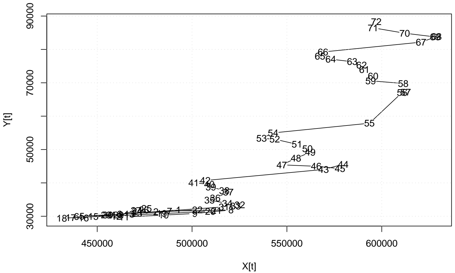
Scatter Plot
