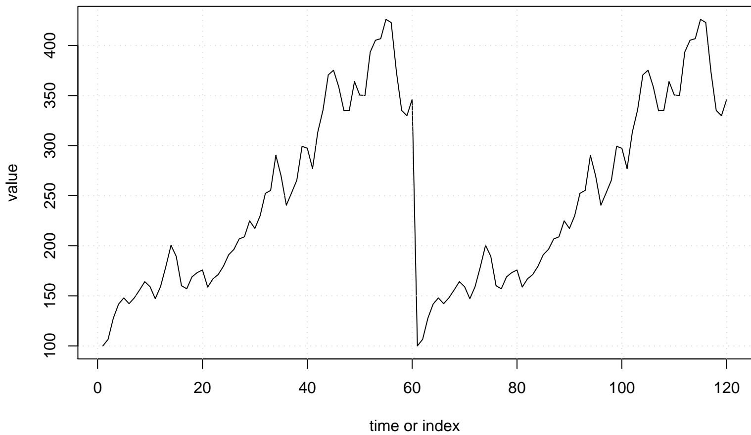
Run Sequence Plot of X[t]
