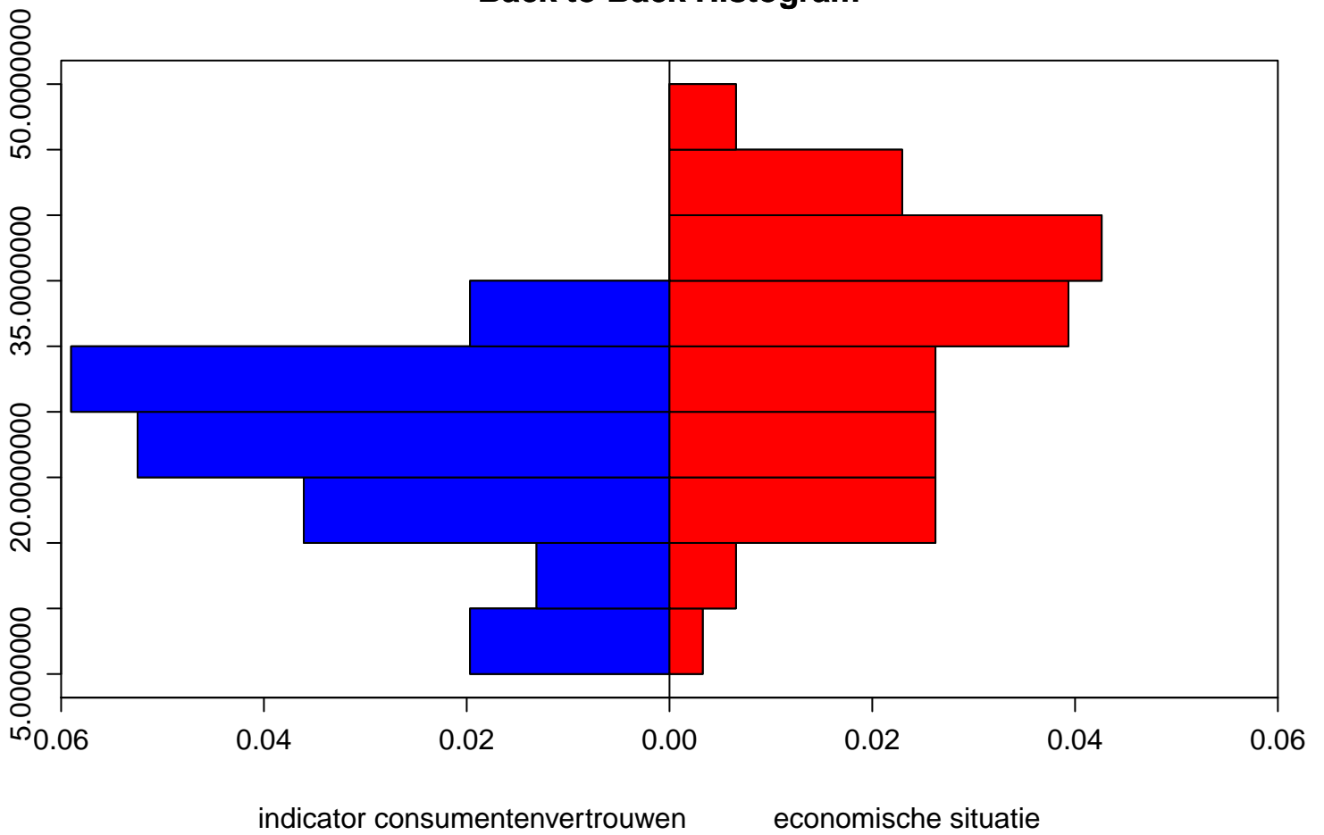
Back to Back Histogram
