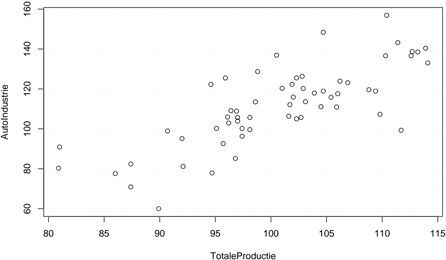
Scatterplot
