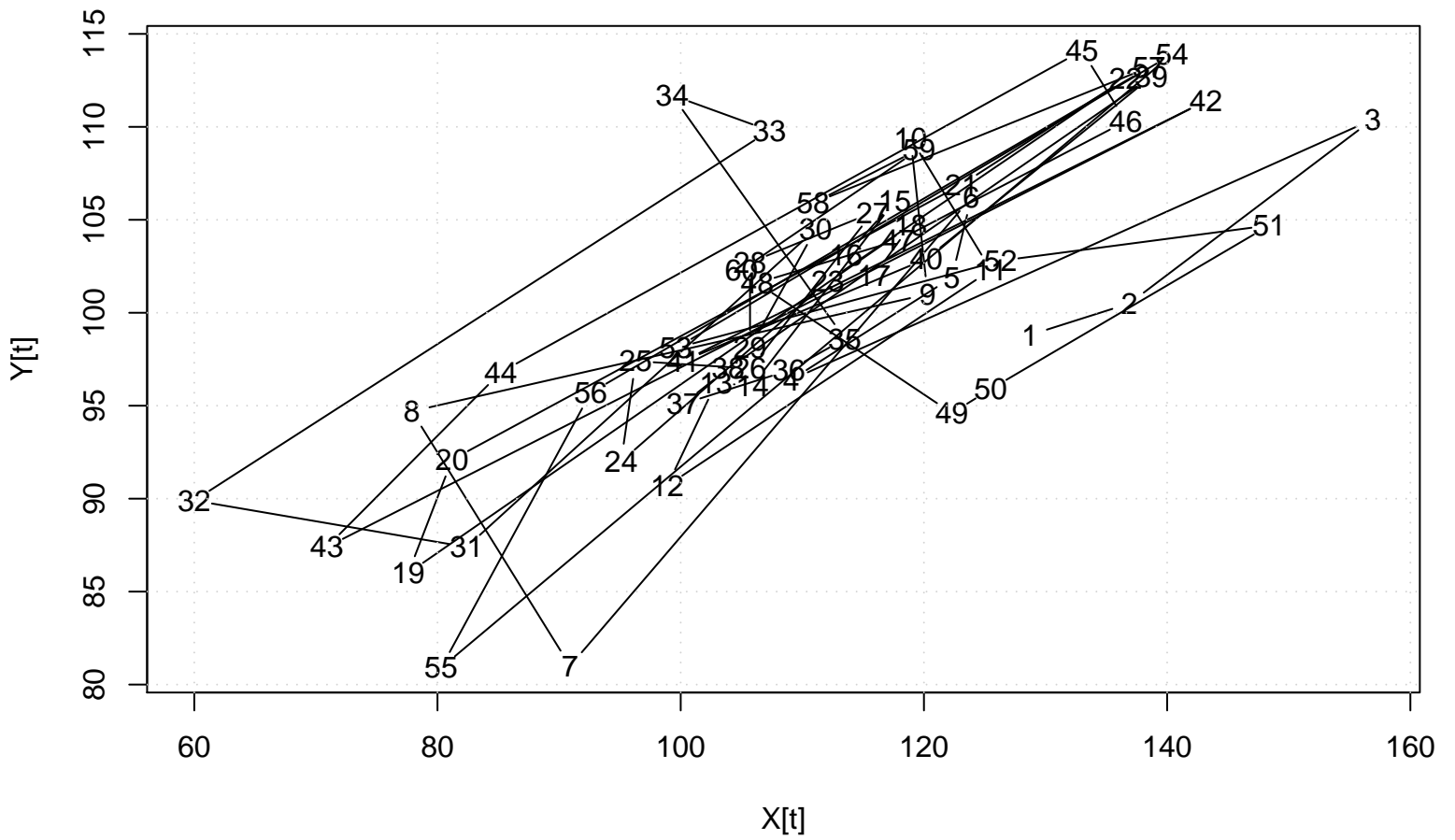
Scatter Plot
