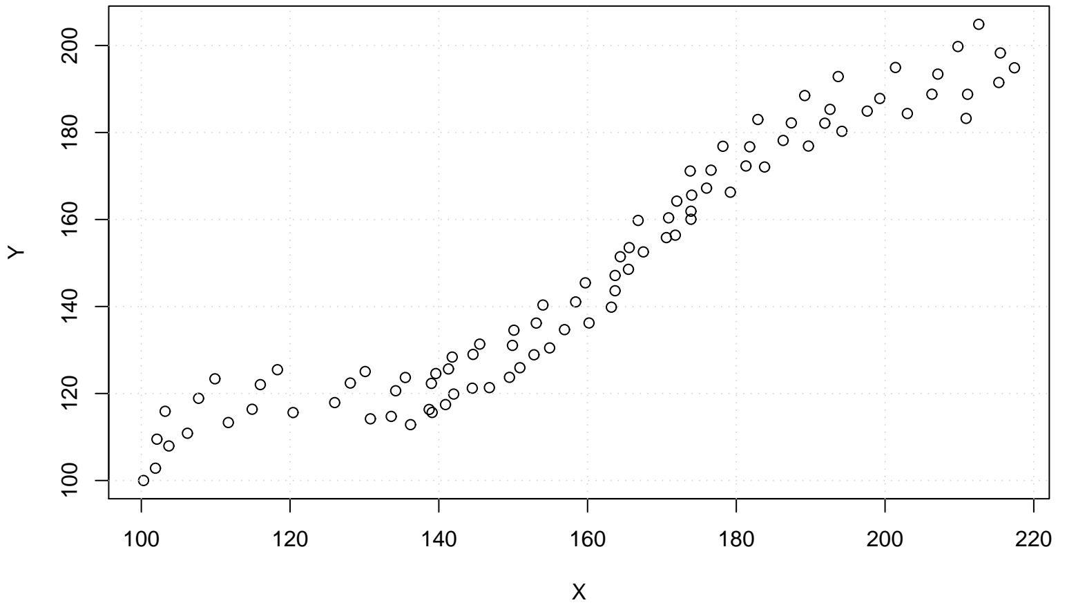
Scatterplot
