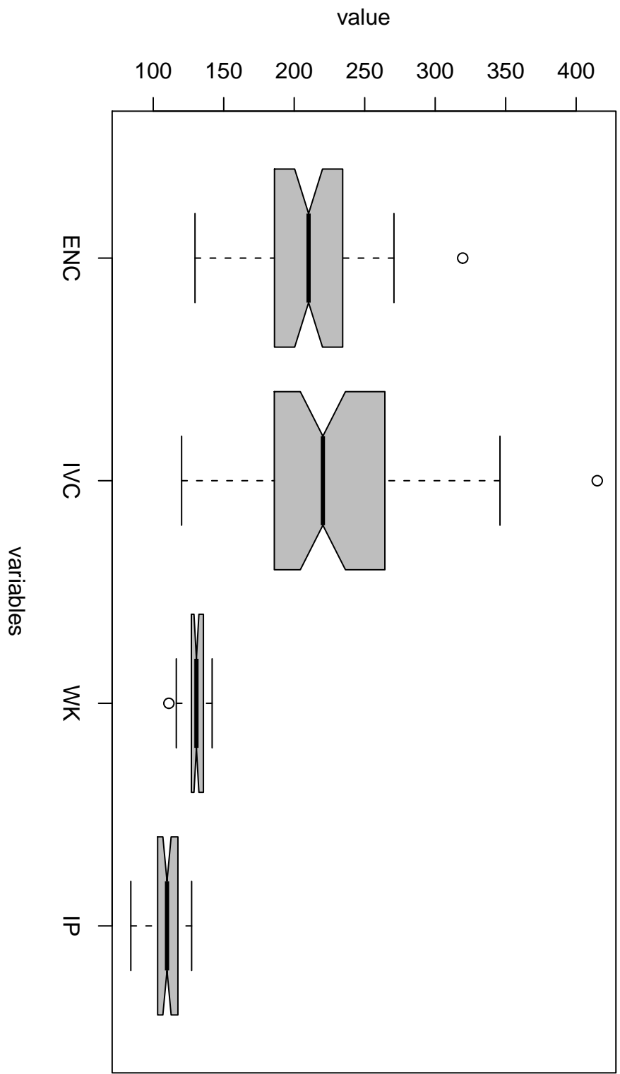
Notched Boxplots
